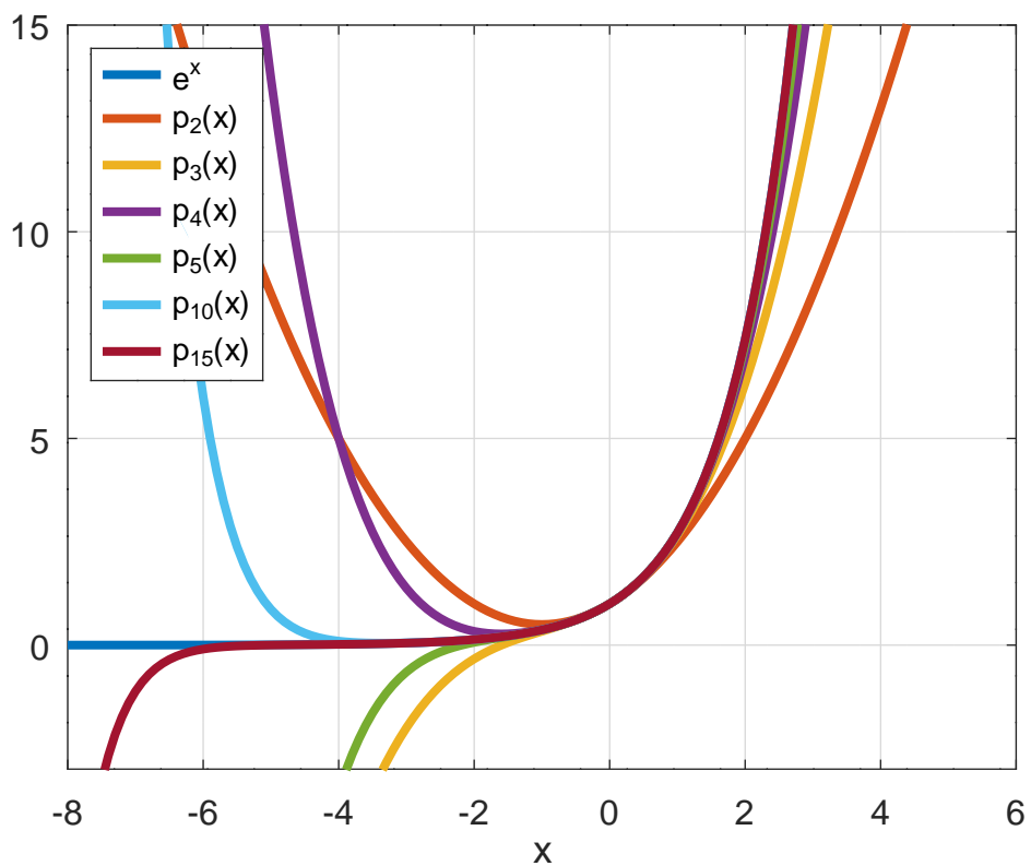
Taylor polynomials approximate e^x
