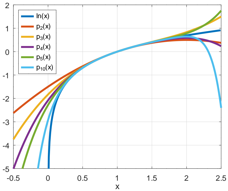
Taylor polynomials approximate \ln(x)
